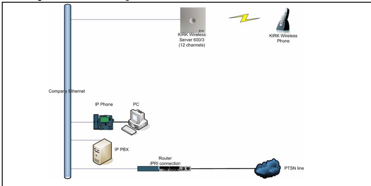
Figure 32 KWS600v3 Single-cell installation
